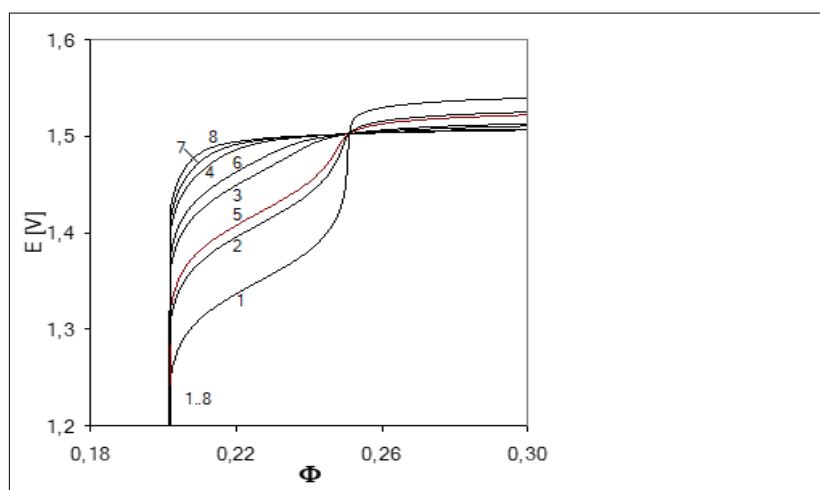
Figure 3. Fragments of hypothetical titration curves plotted for different pairs of stability constants ( K_{31} , K_{32} ) of the complexes \text{Mn}(\text{SO}_4)_i^{+3-2i} : 1 ( 10^4 , 10^7 ); 2 ( 10^3 , 10^6 ); 3 ( 10^{2.5} , 10^5 ); 4 ( 10^2 , 10^4 ); 5 ( 10^4 , 0); 6 ( 10^3 , 0); 7 ( 10^2 , 0); 8 (0, 0); [\text{Mn}(\text{SO}_4)_i^{+3-2i}] = K_{3i}[\text{Mn}^{+3}][\text{SO}_4^{2-}]^i .
