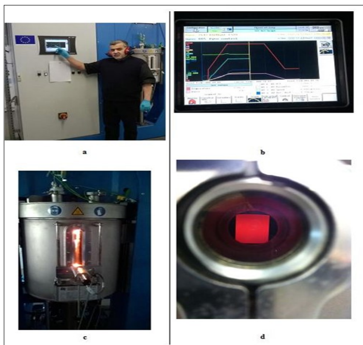
Figure 1. SINTER-LAB, FCT-HP D 25, PS-1050, ENSICAEN. (a)-The author, (b)-Variation of the displacement, the displacement rate and the temperature in dependence of the heating time, (c, d)- The plasma produced by the current in the SPS chamber.
