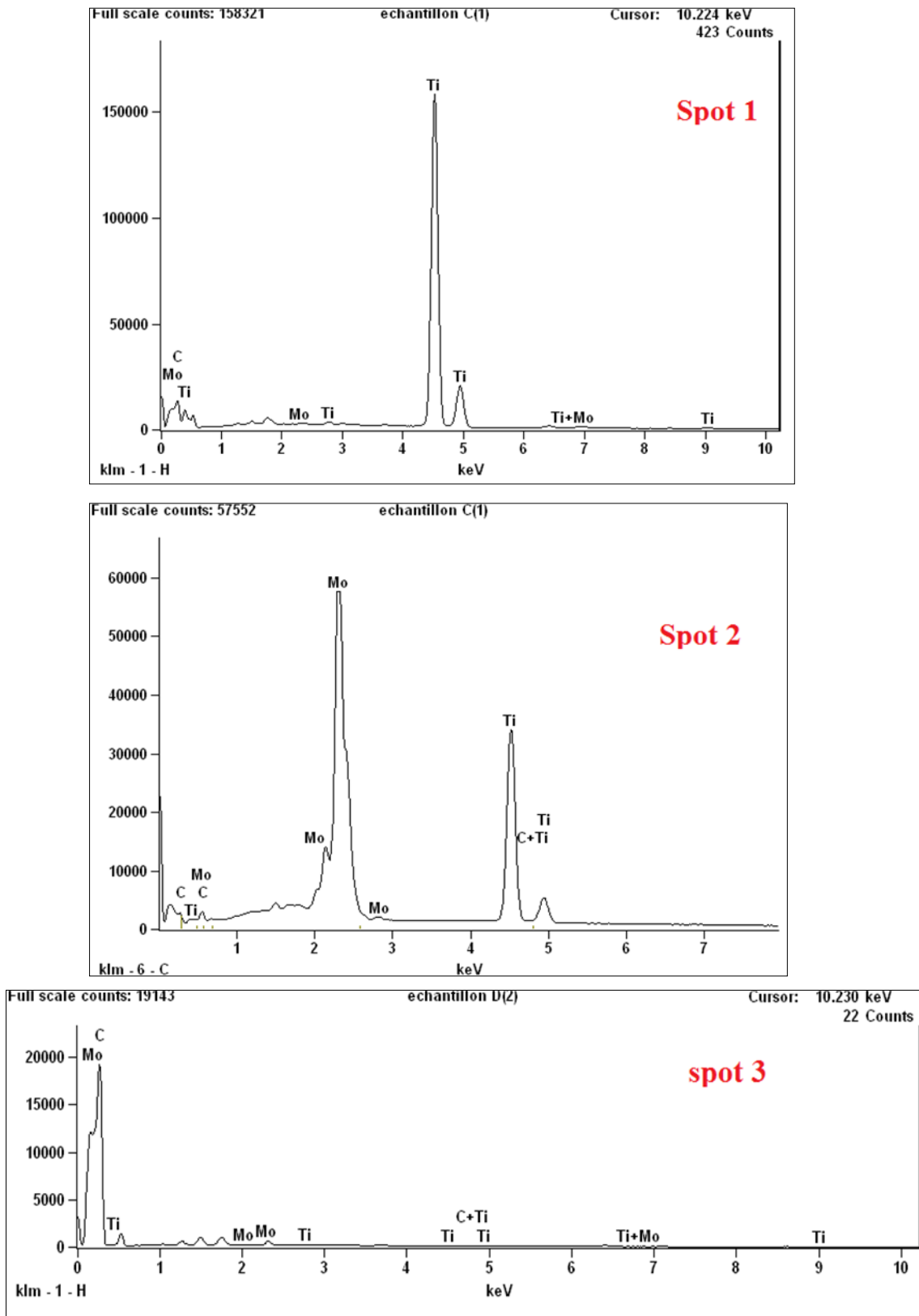
Figure 5. EDX spectra in different regions of MTC polished and etched surface for the sintered samples using a 20-mm diameter die: (Spot1)- TiC regions , (Spot2)-Mo 2 C regions , (Spot3)-SWCNTs regions
