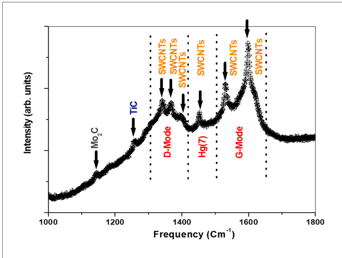
Figure 10. Raman spectra of the synthesized samples using a 20 mm diameter die.
