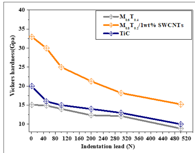
Figure 6. Representation the variation of Vickers microhardness function of the indentation lead of MTC polished and etched surface for the sintered samples using a 20 mm diameter die
