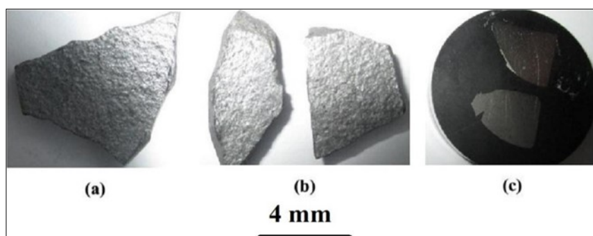
Figure 2. Images of sintered MTC: (a, b) coarse grinding; (c) fine polishing.
