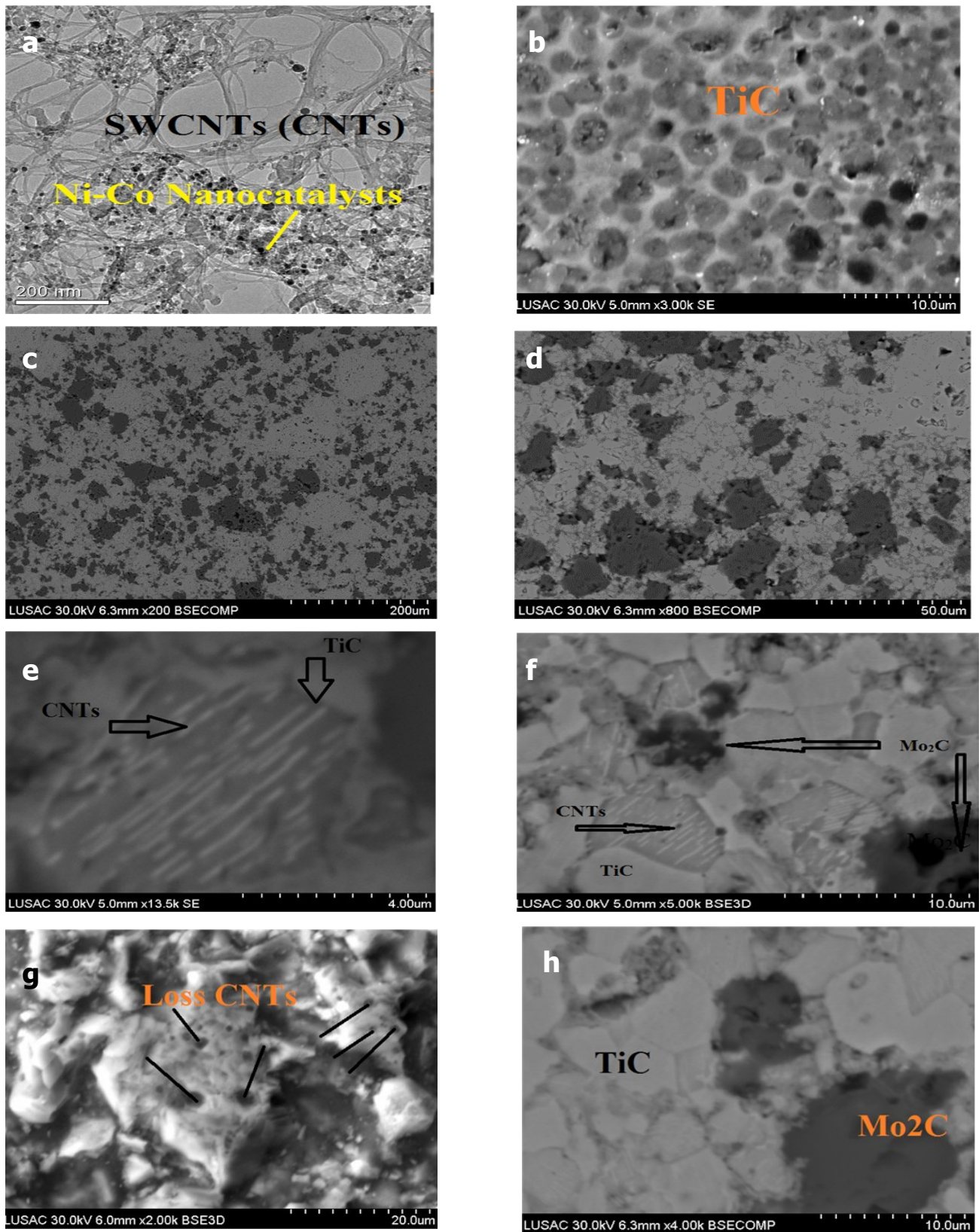
Figure 3. High magnification microstructural representative SEM image of MTC polished and etched surface for the sintered samples using a 20-mm diameter die. (a)-TEM of SWCNTs , (b)-Sintered TiC grains, (c)-Nanocomposites overview, (d)- nanocomposites overview with magnification, (e)- SWCNTs into the TiC grain, (f)- SWCNTs into the TiC grains, (g)-Pore like structure of losses SWCNTs , (h)-Nanocomposites overview with higher magnification.
