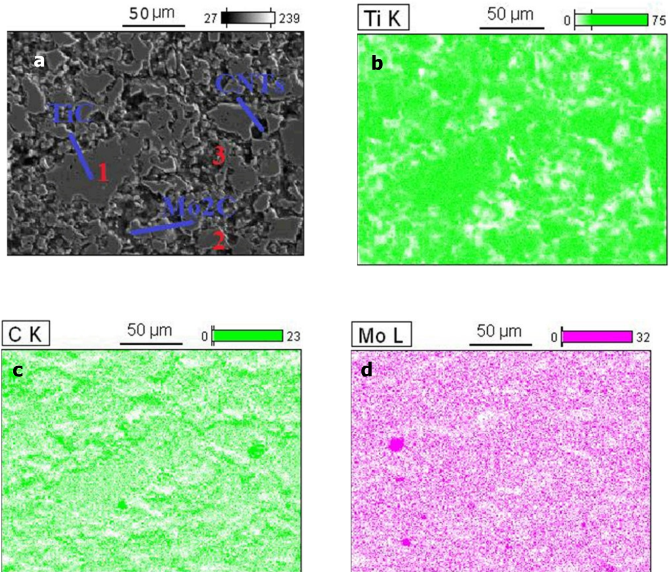
Figure 4. Microstructural representation and EDS maps of MTC analysis displays elemental analyses of the various regions of the sintered samples. Secondary electron image, atomic concentration cartographies of Mo, Ti, and C of MTC polished and etched surface for the sintered samples using a 20-mm diameter die. :(a)- Overview of the nanocomposite , (b)- Cartographies of Ti, (c)- Cartographies of C, (d)- Cartographies of Mo.
