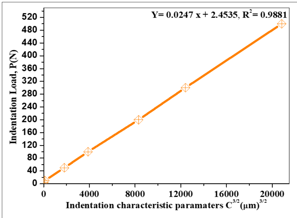
Figure 9. Correlation in between the applied load P, and half-length of median crack c^{3/2} of MTC polished and etched surface for the sintered samples using a 20 mm diameter die
