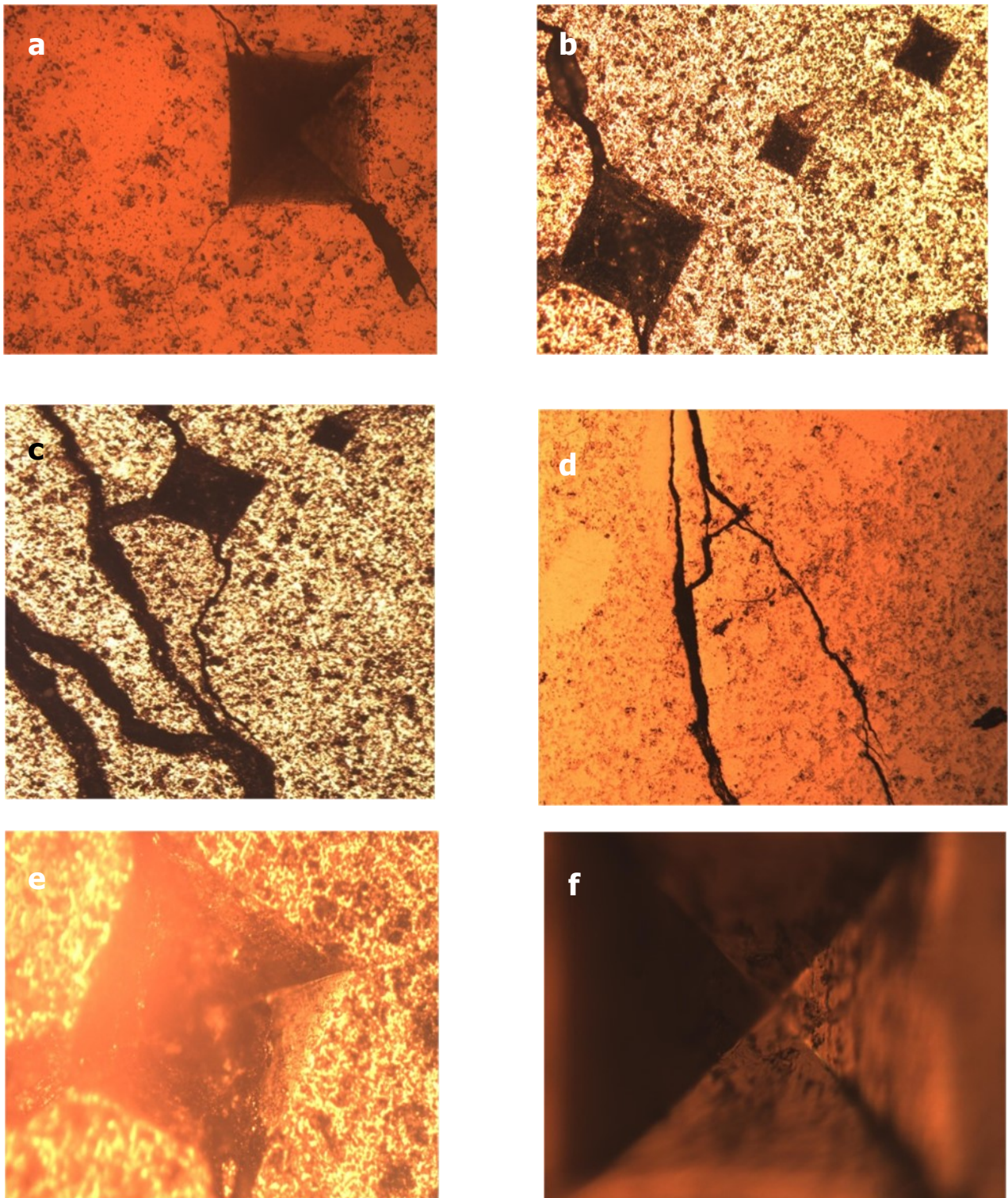
Figure 8. Optical micrograph of crack patterns used for IFT calculations of (a, b)-MTC tested at 300 N, (c)-MTC tested at 500 N. Micrographs of cracks at the corners of Vickers indentation: (d)-Etched MTC showing a purely transgranular crack growth and (e, f)-High magnification of indentation label.
